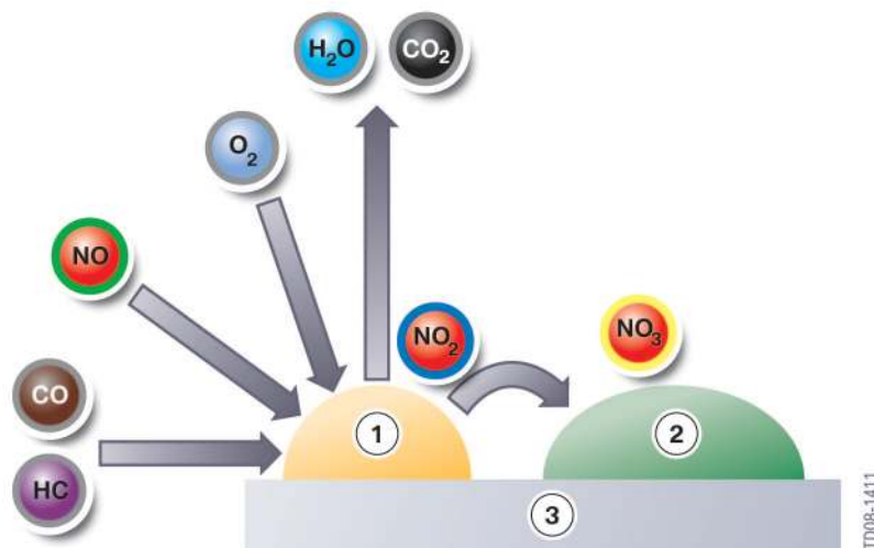
52 - NO x storage
