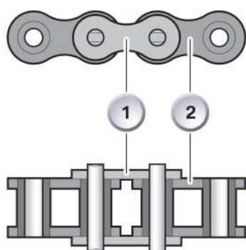
28 - Bush chain
