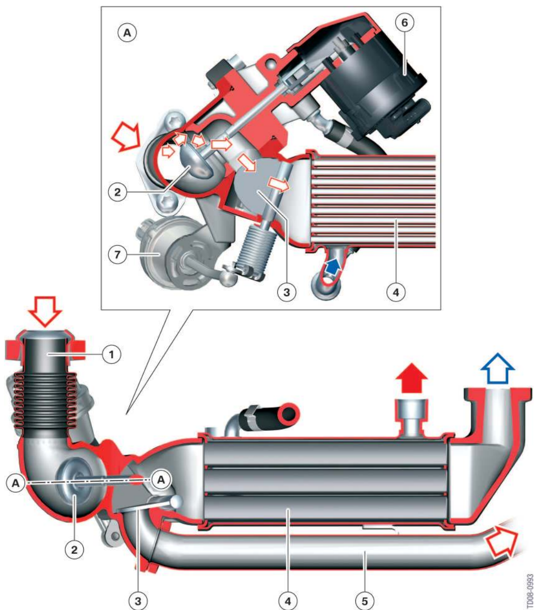
65 - EGR cooler with bypass
