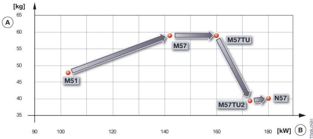
6 - Development of crankcase weight and engine output
