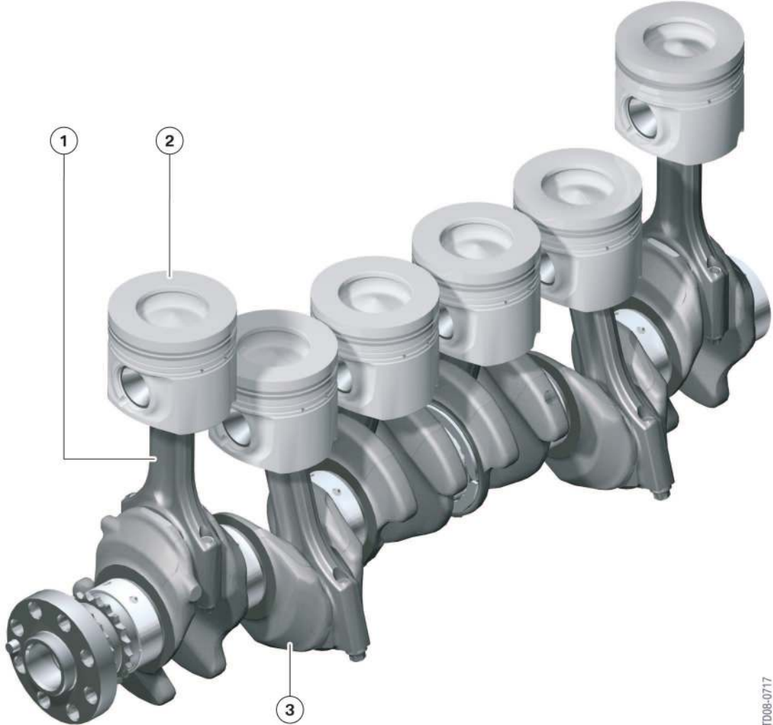
2 - Crankshaft drive system, N57 engine
