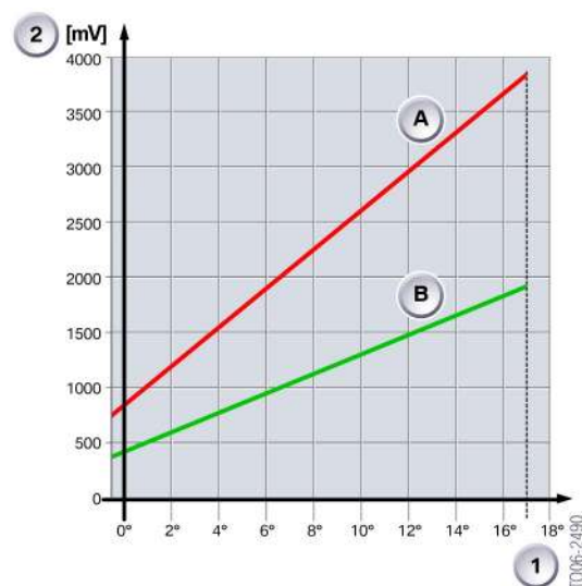
104 - Signal progression of accelerator pedal module
