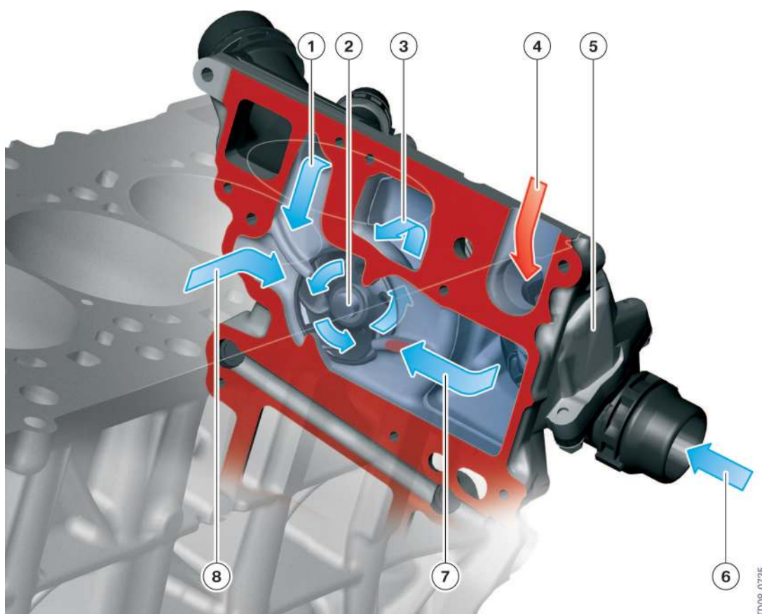
89 - Coolant pump, N57 engine
