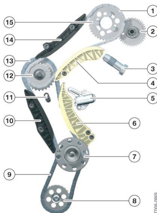
27 - Chain drive system, N57 engine
