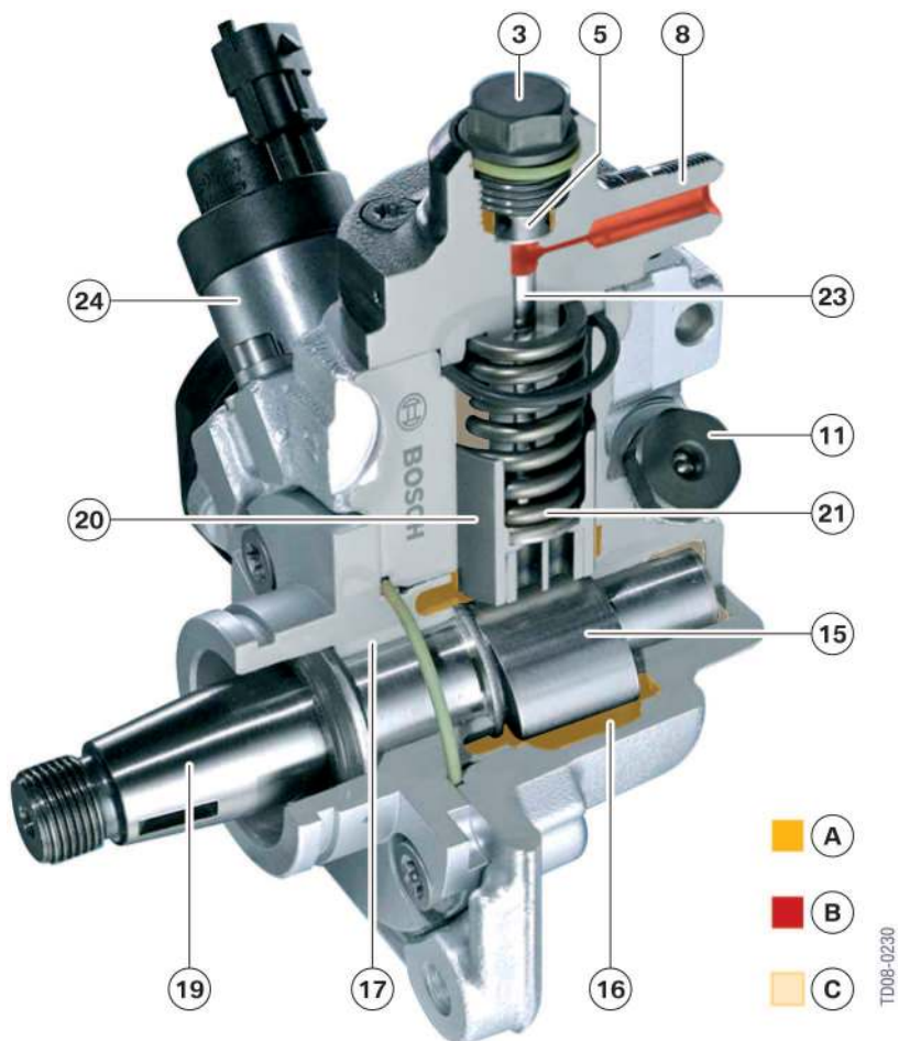
82 - High-pressure pump CP4.2
