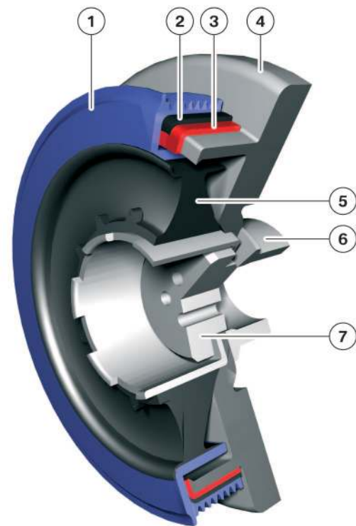
26 - Rotational vibration damper
