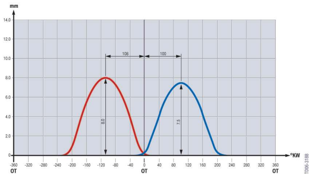
5 - Timing graph, N57 engine
