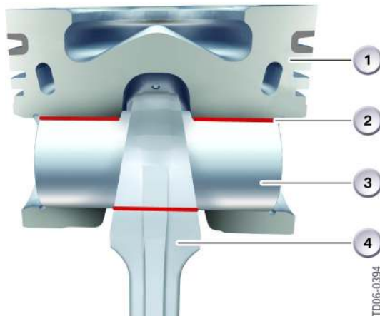
21 - Trapezoidal connecting rods
