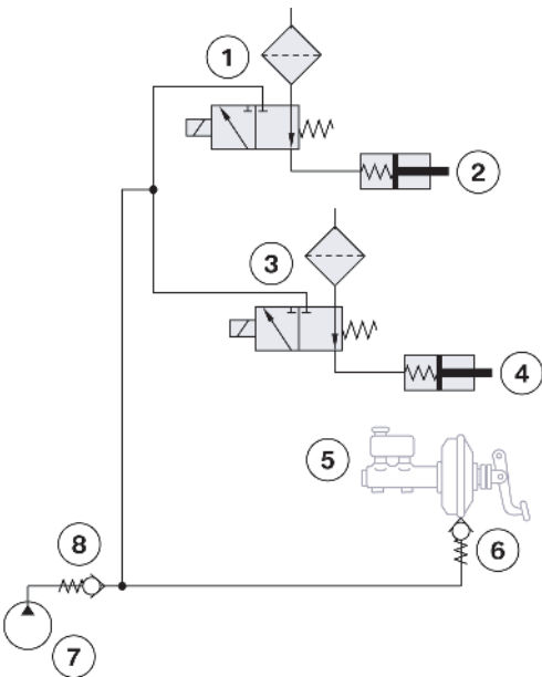
67 - Vacuum system, N57 engine
