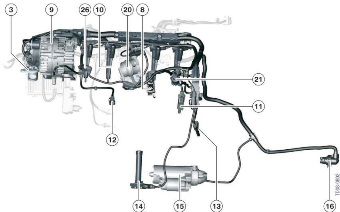
94 - Wiring loom on N57 engine in F01, view from left
