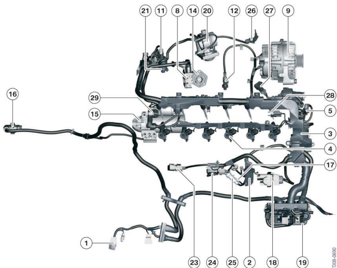
96 - Wiring loom on N57 engine in F01, top view
