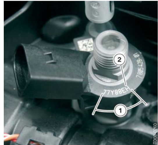
85 - Piezo-electric injector volume calibration code
