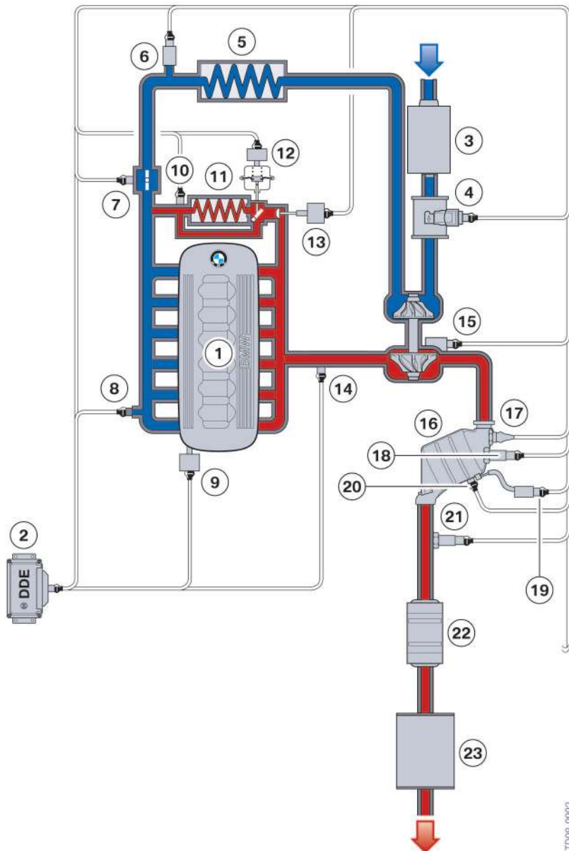
45 - Air intake and exhaust system on N57 engine for EURO 6 on E90
