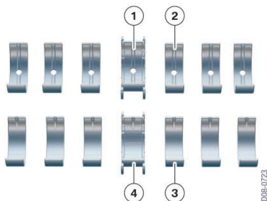
19 - Crankshaft bearings, N57 engine
