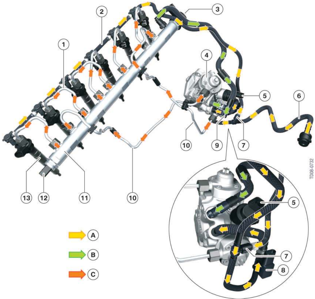
78 - Common-rail system with piezo-electric injectors on N57D30 O0 engine
