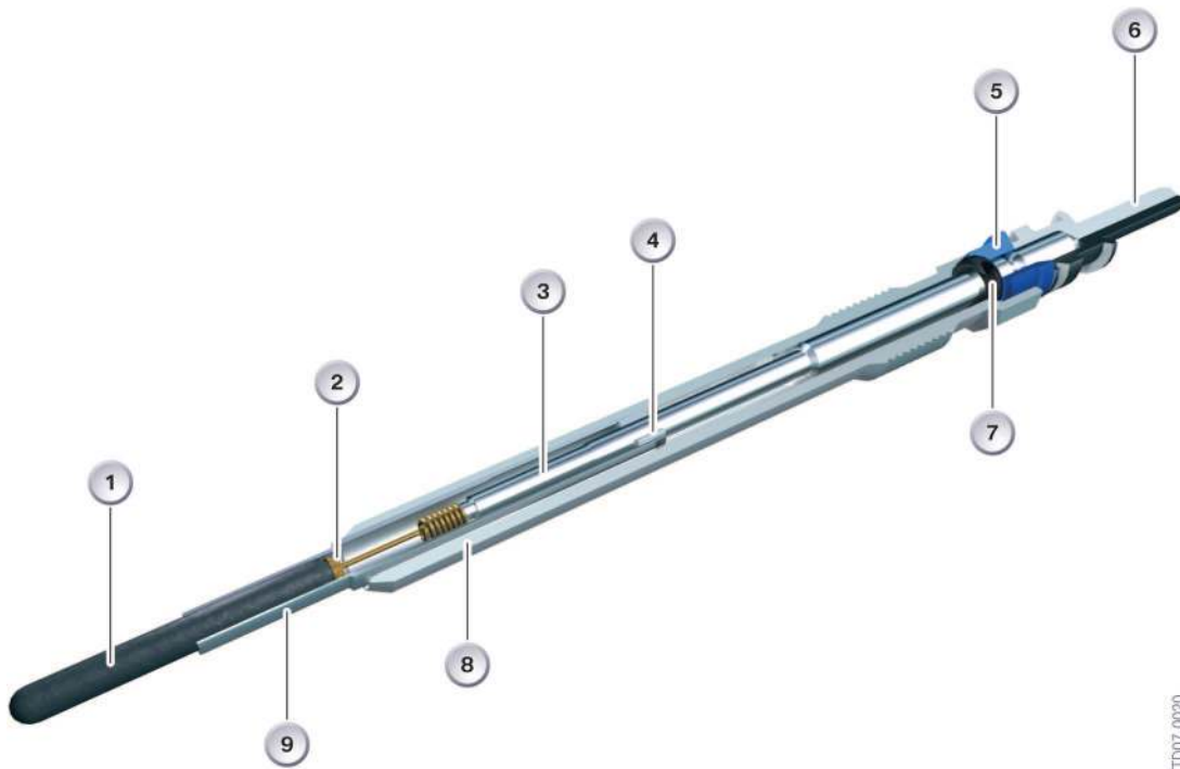
150 - Glow plug
