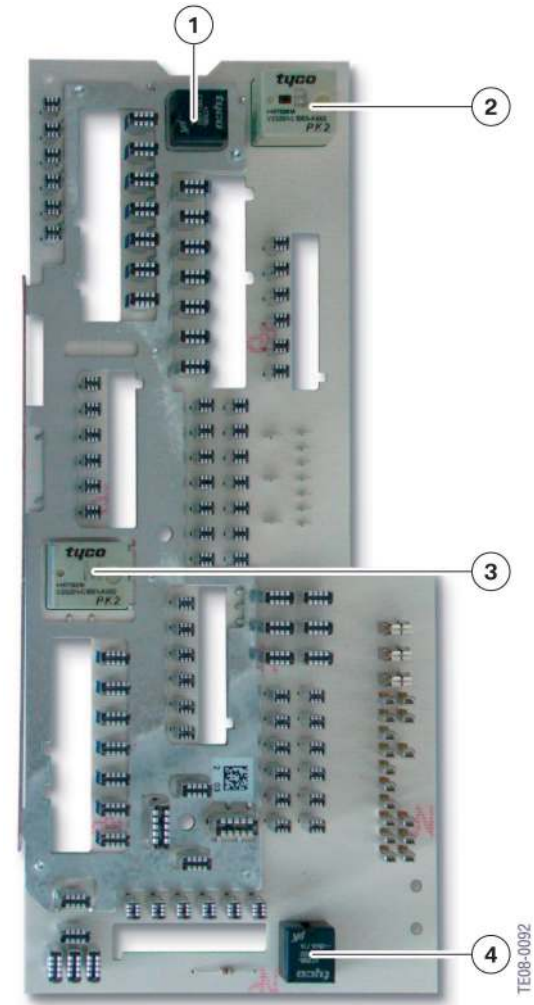
129 - Front fuse box on F01/F02
