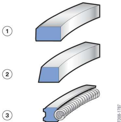
23 - Piston ring set, N57 engine
