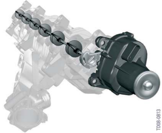
145 - Swirl flap regulator
